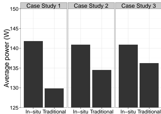
Fig. 8: Average power of post-processing and in-situ pipelines
