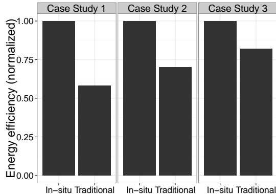
Fig. 11: Energy efficiency of post-processing and in-situ pipelines
