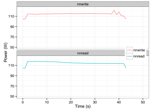
Fig. 6: Power profile of nnread and nnwrite stages
