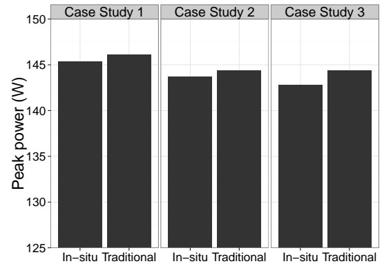
Fig. 9: Peak power of post-processing and in-situ pipelines
