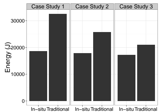
Fig. 10: Energy consumption of post-processing and in-situ pipelines
