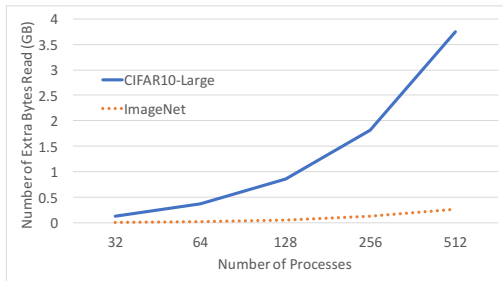
Fig. 10. Caffe/LMDBIO-LMM: Extra bytes read
