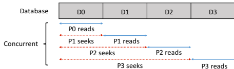
Fig. 5. LMDB redundant data movement
