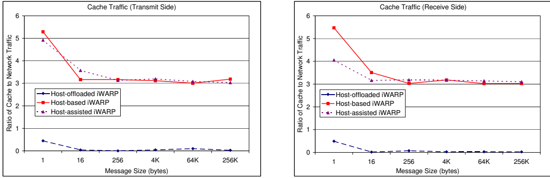
Fig. 12. iWARP Out-of-Cache Communication Bandwidth: (a) Transmit Side, (b) Receive Side
