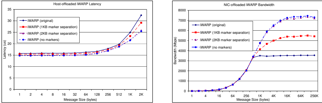
Fig. 13. Impact of marker separation on iWARP performance: (a) Latency (b) Bandwidth
