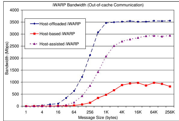
Fig. 11. Out-of-Cache Communication
